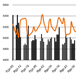
FTSE 100 INDEX
